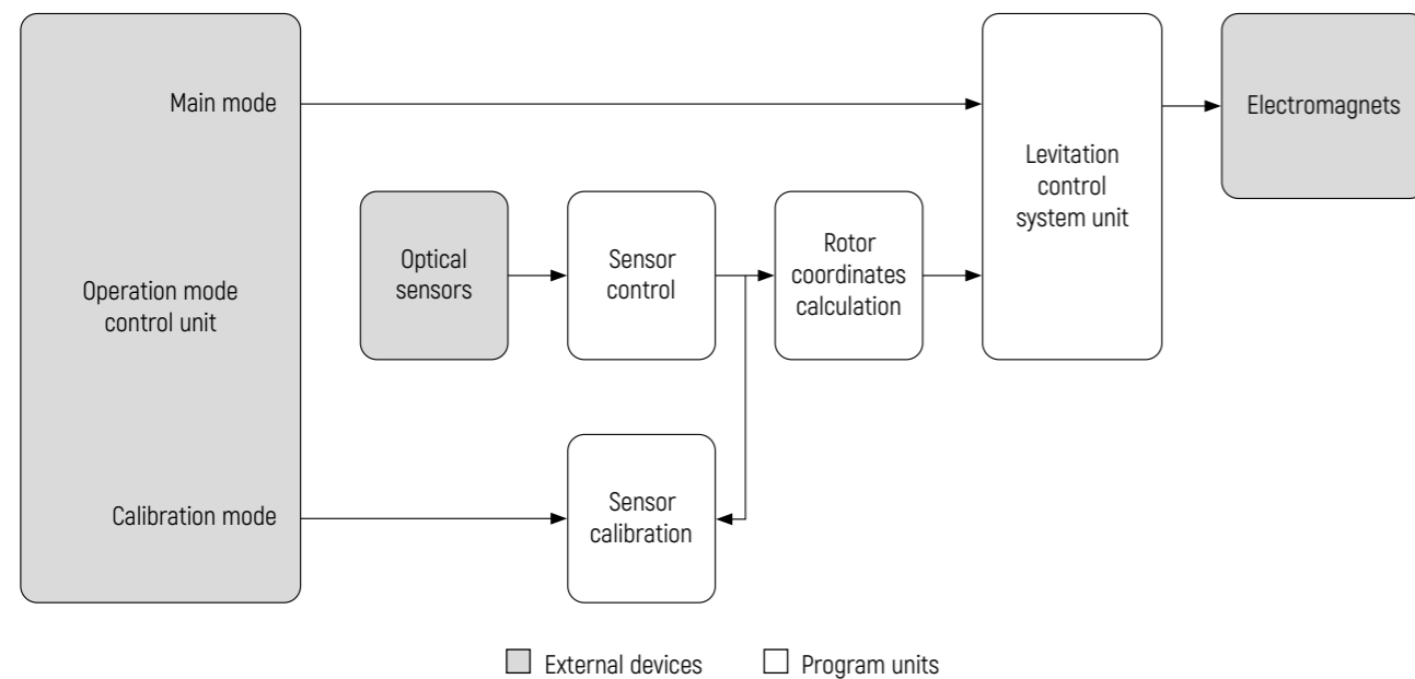
Figure 7 - Flowchart of the stabilization control system
