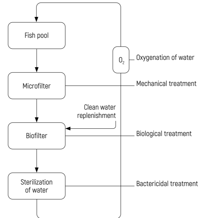
Figure 10 – Structure of the fishery recirculation system
