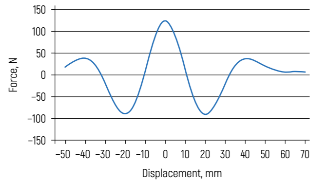
Figure 26 – Dependence graph of force on the displacement of one two-dimensional Halbach array relative to another
