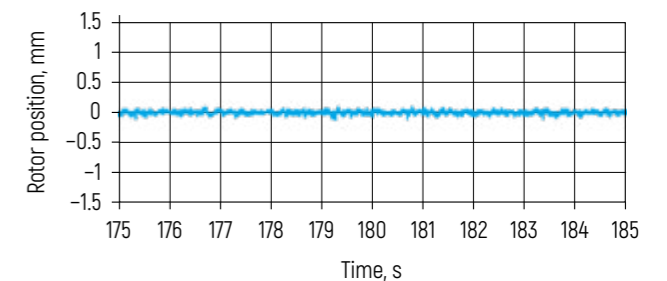
Figure 16 – Rotor stabilization after displacement from the equilibrium point
