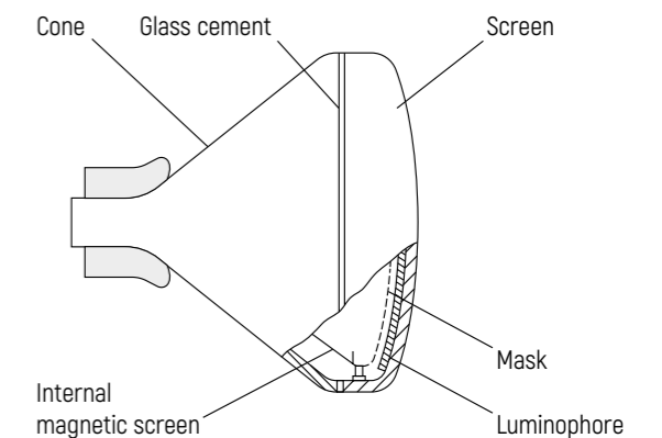
Figure 2 – Components of the kinescope
