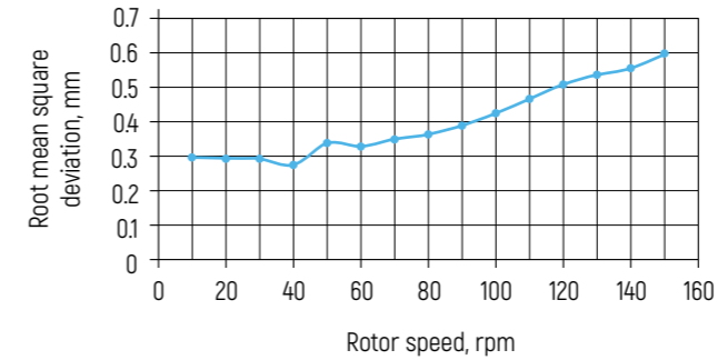
Figure 21 – Measured transverse vibrations of the rotor at different rotation speeds
