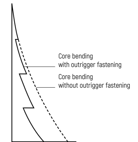
Figure 24 - Epure of moments of the stiffening core with outriggers from the wind impact
