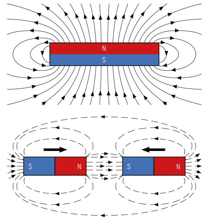
Figure 1 – Shape of fields of a single and sequentially arranged magnets
