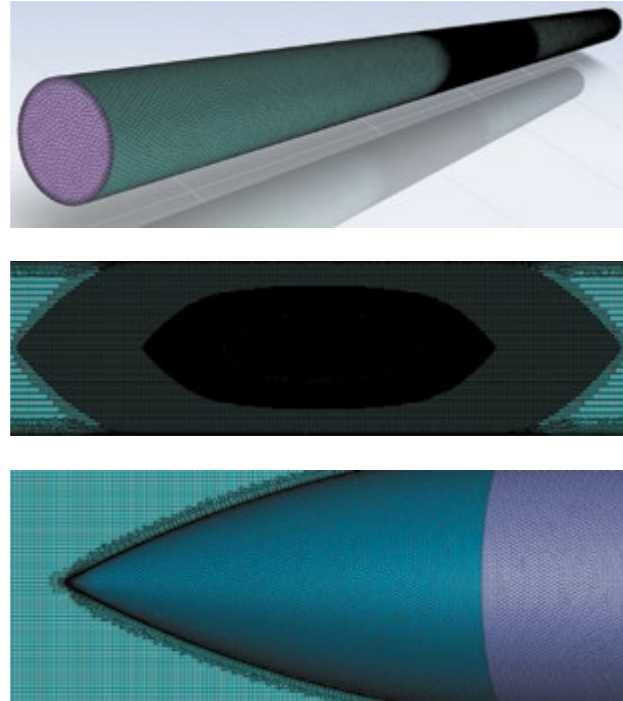
Figure 3 – Finite element model
