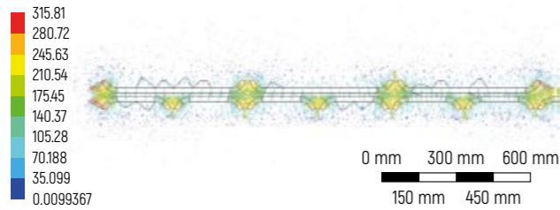
Figure 11 – Magnetic flux distribution in the initial position at rotor magnets length of 575 mm, mT
