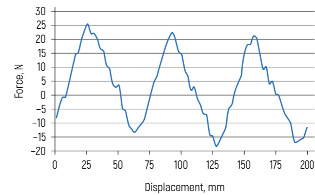
Figure 28 – Dependence graph of longitudinal force of resistance to rotor motion on its displacement at rectangular shape of magnets
