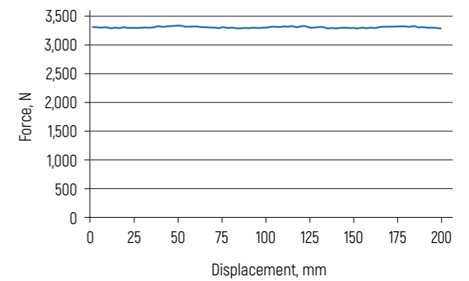
Figure 31 – Dependence graph of lifting force on rotor displacement at vaulted shape of magnets
