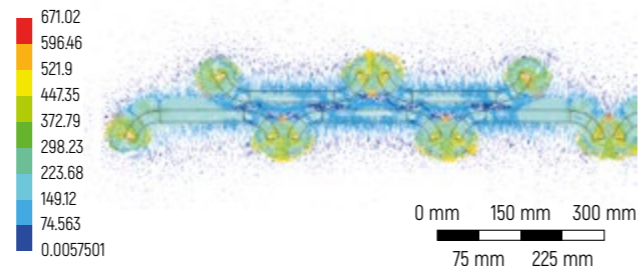
Figure 5 – Magnetic flux distribution at longitudinal displacement of rotor magnets relatively to stator magnets by 160 mm, mT
