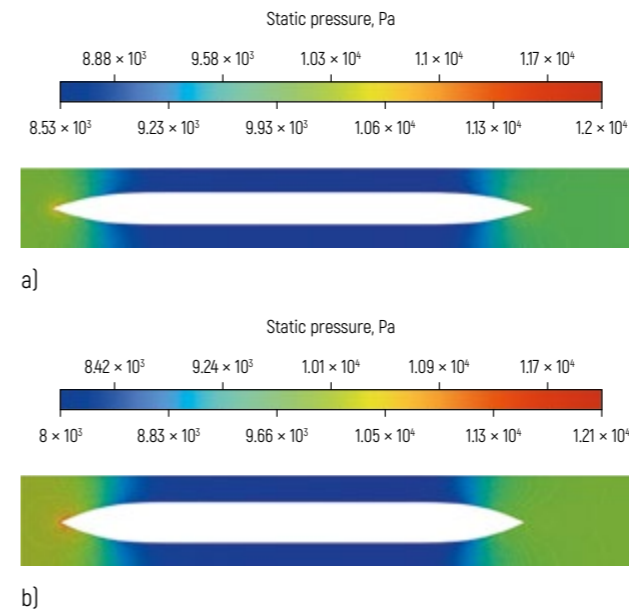
Figure 5 – Distribution of pressure in the volume of methane gas medium: a – for uPod fuselage diameter of 2 m and tunnel inner diameter of 5 m; b – for uPod fuselage diameter of 2.6 m and tunnel inner diameter of 6 m
