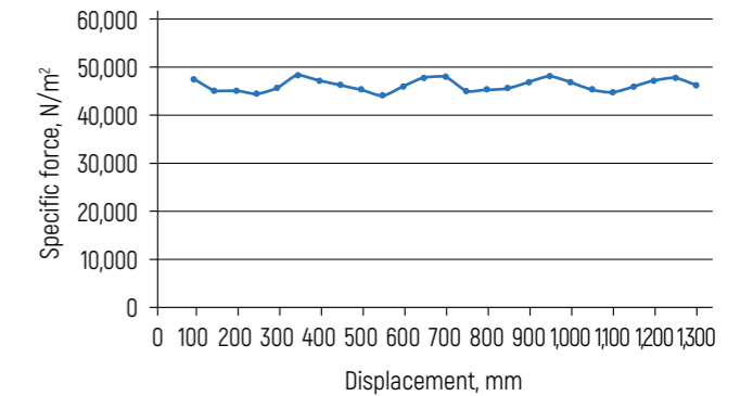
Figure 17 – Dependence graph of the specific interaction force between stator and rotor on their mutual displacement at rotor magnets length of 575 mm
