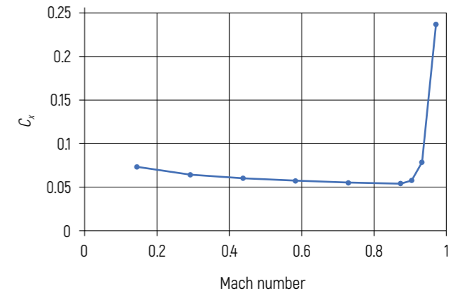
Figure 1 – Diagram of dependence of aerodynamic drag coefficient C x on Mach number for the hypervelocity uPod when moving in atmospheric air
