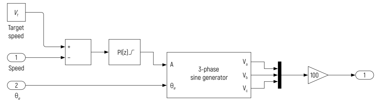
Figure 13 – Control unit
