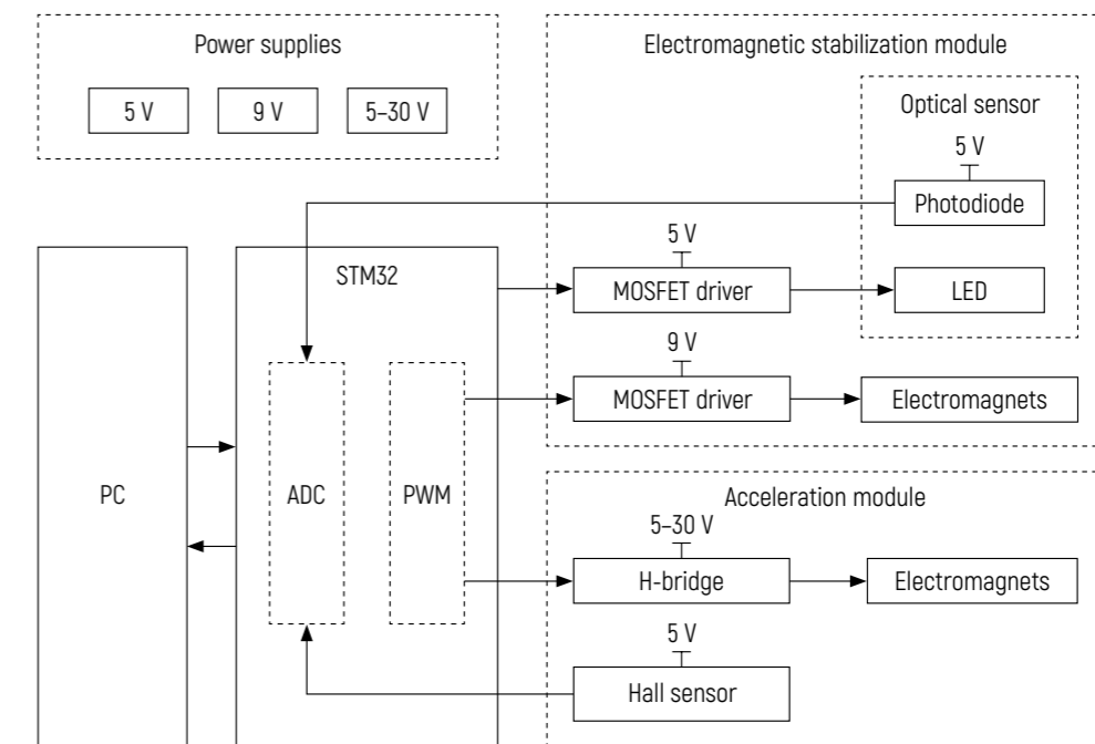
Figure 4 – Structural diagram of the test bench
