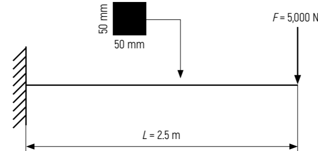
Figure 7 – Calculation diagram of problem 3. Cantilever beam (dynamic positioning)
