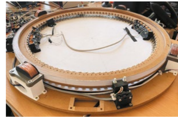
Figure 3 – Experimental test bench developed by Unitsky String Technologies Inc. (Minsk, 2023)
