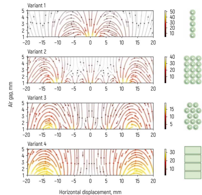
Figure 6 – Variants of stator magnet configurations (right). Vector maps of repulsive forces (left)
