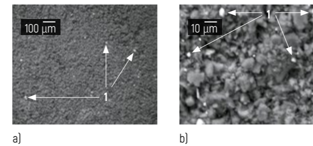
Figure 4 – Electron-microscopic images of brown coal sample structure (initial fraction of 3–5 mm) with particle size less than 100 μm after grinding for 10 min: a – 100 times magnification; b – 1,000 times magnification; 1 – inclusions of mineral content
