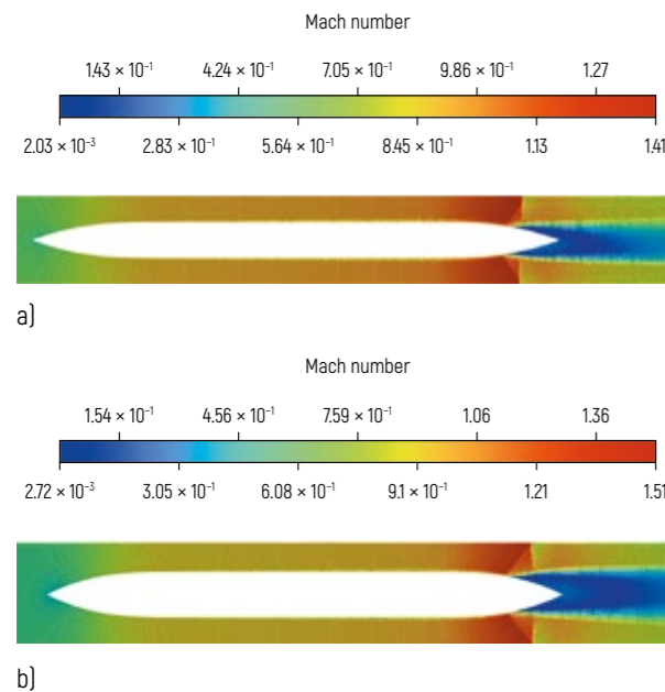
Figure 7 – Distribution of Mach number of air gas medium in a forevacuum tunnel: a – for uPod fuselage diameter of 2 m and tunnel inner diameter of 5 m; b – for uPod fuselage diameter of 2.6 m and tunnel inner diameter of 6 m
