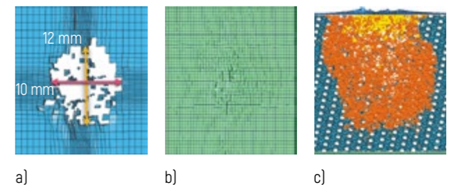
Figure 10 – Results of the computational experiment on penetration of the protective panel: a – front wall; b – rear wall; c – foam aluminum
