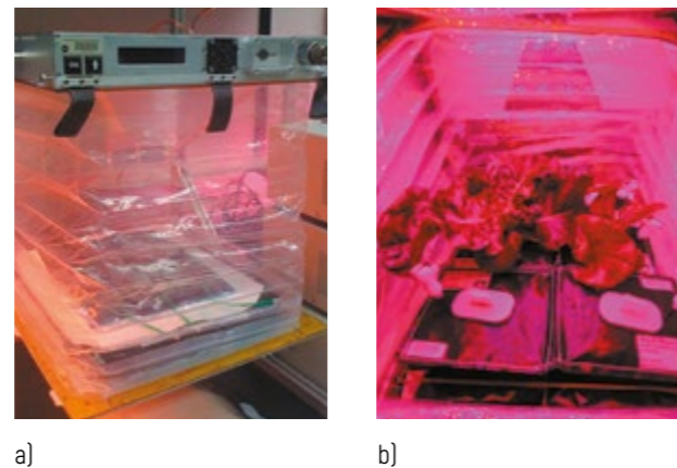
Figure 2 – Veggie vegetable growing system: a – terrestrial prototype before the launch [8]; b – Veg-03 version in operation [9]
