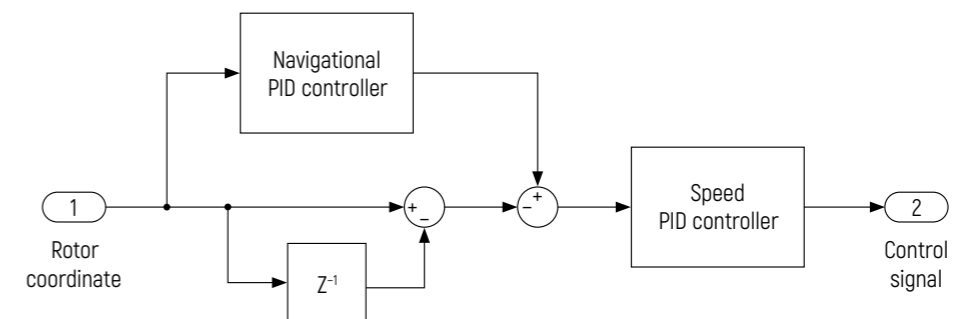
Figure 10 - Controllers of the levitation control system unit
