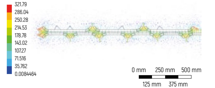
Figure 8 – Magnetic flux distribution in the initial position at rotor magnets length of 500 mm, mT
