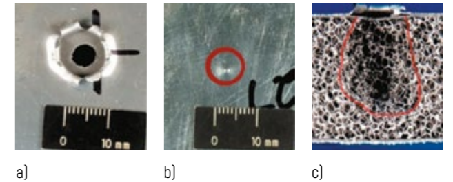
Figure 9 – Results of the HITF-08263 field experiment on penetration of the protective panel: a – front wall; b – rear wall; c – foam aluminum
