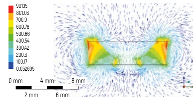
Figure 5 – Distribution of magnetic induction field of the magnet, mT
