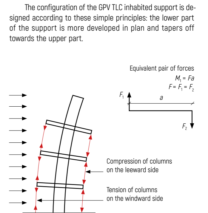
Figure 20 – Diagram for determining the equivalent pair of forces
