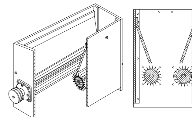
Figure 3 – Rotary crusher
