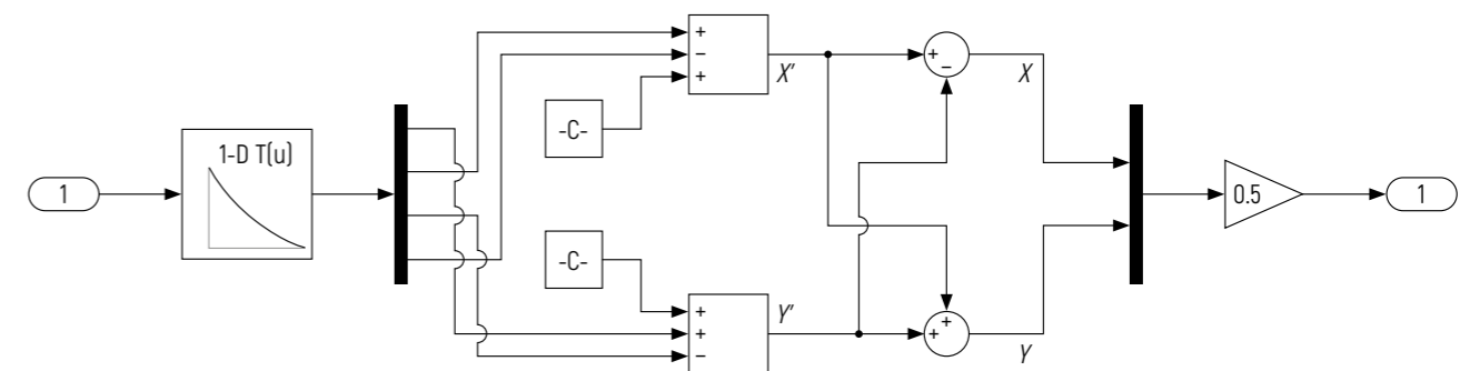
Figure 9 - Rotor coordinate calculation unit
