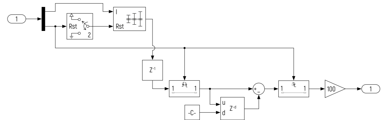
Figure 8 - Optical sensor control unit
