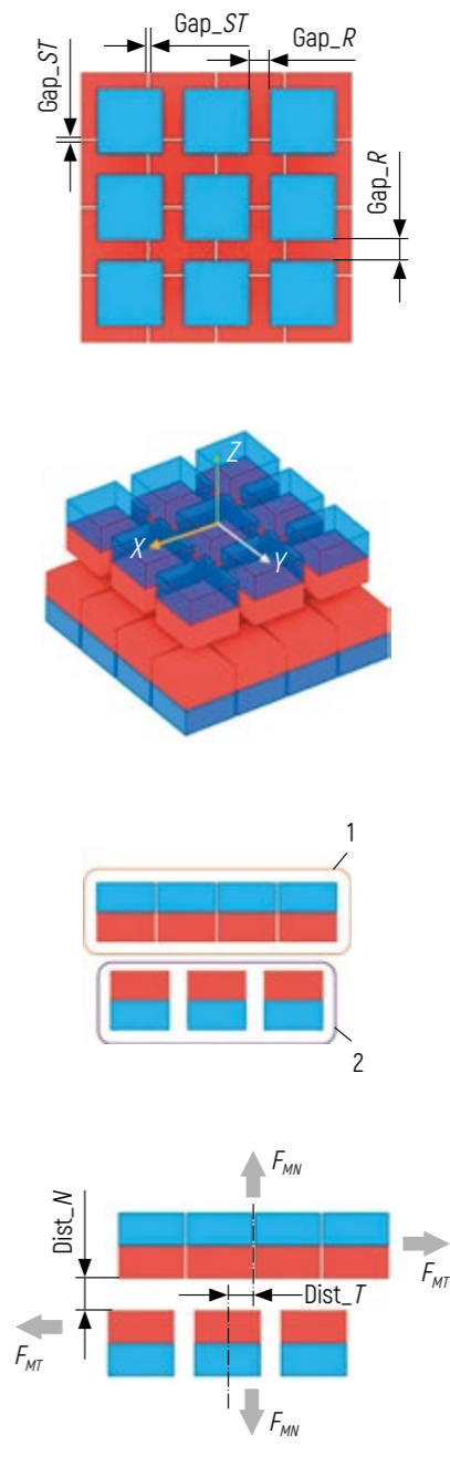
Figure 2 – Construction of a magnetic assembly power unit made of discrete neodymium magnets: a – top view; b – isometric view; c – side view at the nominal position of the magnetic groups; d – side view at the tangential displacement of the magnetic groups; 1 – stator magnetic group; 2 – rotor magnetic group
