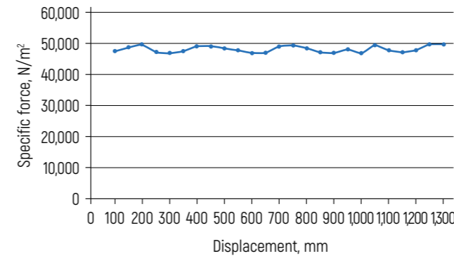
Figure 16 – Dependence graph of the specific interaction force between stator and rotor on their mutual displacement at rotor magnets length of 500 mm
