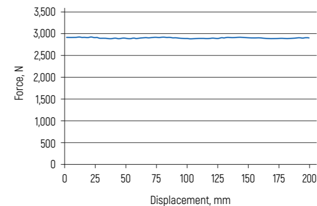
Figure 30 – Dependence graph of lifting force on rotor displacement at rectangular shape of magnets
