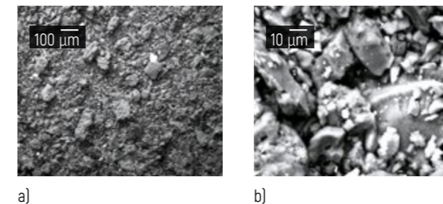
Figure 5 – Electron-microscopic images of brown coal sample structure (initial fraction of 0–50 mm) after grinding for 15 min: a – 100 times magnification; b – 1,000 times magnification
