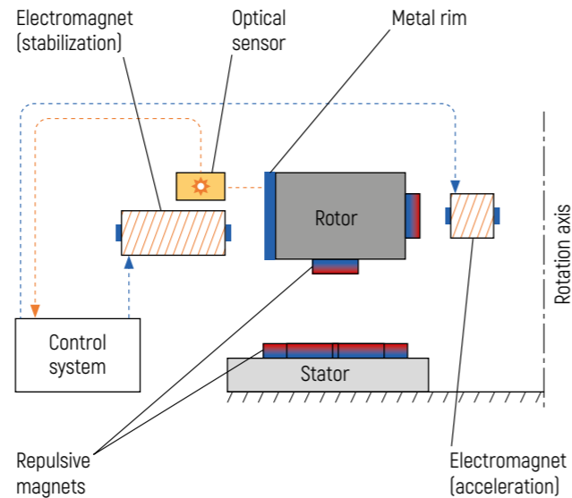
Figure 1 – Functional diagram of the test bench ring model
