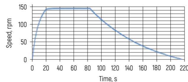
Figure 20 – Result of rotor acceleration and deceleration
