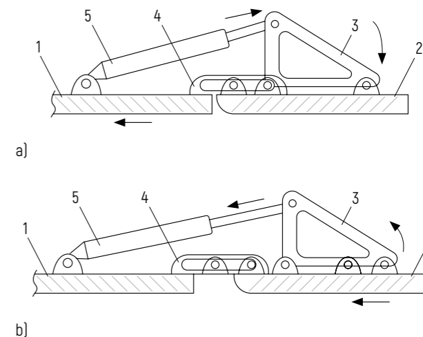
Figure 4 – Design diagram of the mechanism for moving the upper and lower parts of the concrete paver: a – concreting position; b – position of movement of the sliding formwork (moving part); 1 – sliding formwork (moving part); 2 – thrust plate; 3 – lever mechanism; 4 – guide; 5 – hydraulic cylinder
