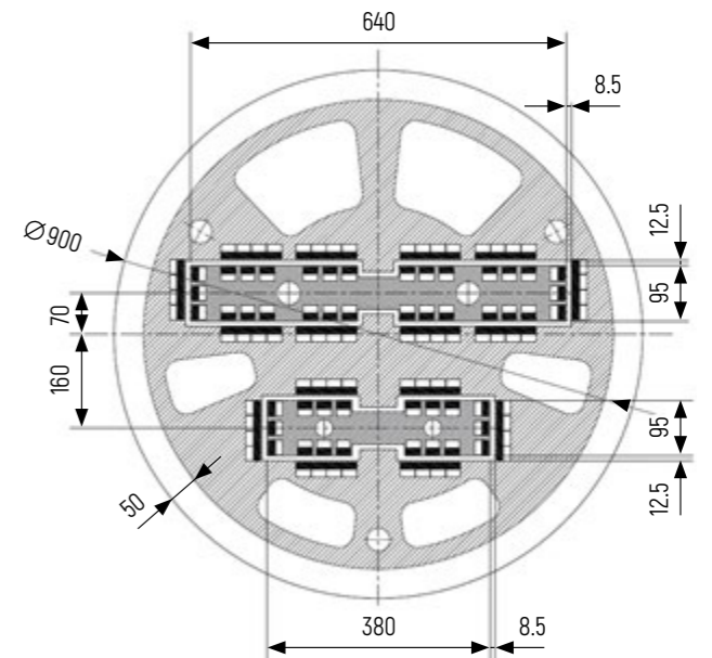
Figure 4 – Cross section of the GPV with the MSSU of linear rotors (option), mm
