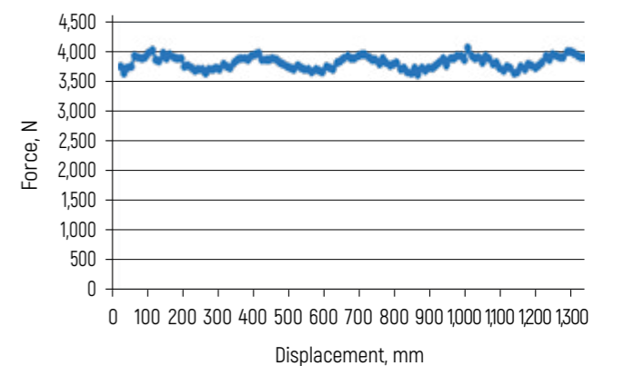
Figure 9 – Dependence graph of force interaction between stator and rotor on their mutual displacement at rotor magnets length of 500 mm
