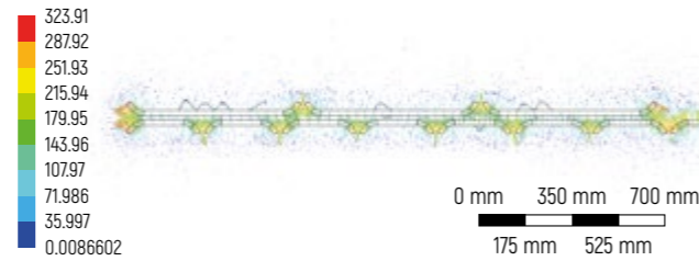
Figure 14 – Magnetic flux distribution in the initial position at rotor magnets length of 650 mm, mT
