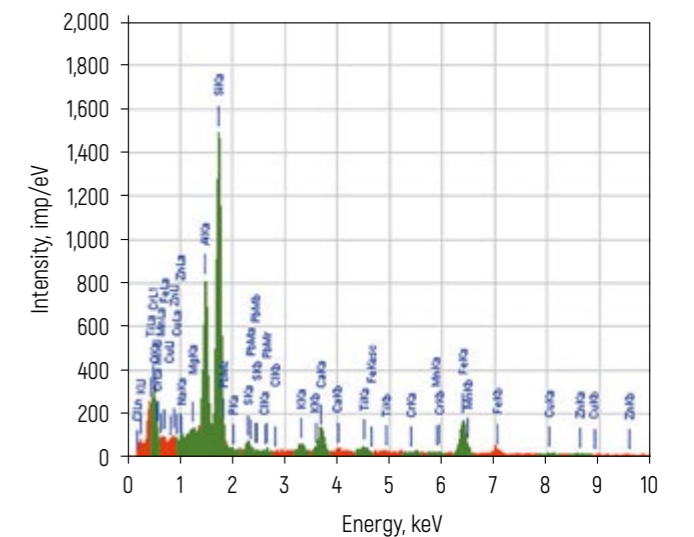
Figure 6 – The result of electron-probe chemical analysis of brown coal ash residue
