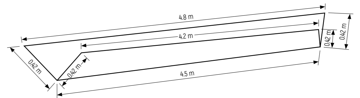
Figure 7 - Diagram of the streambed module
