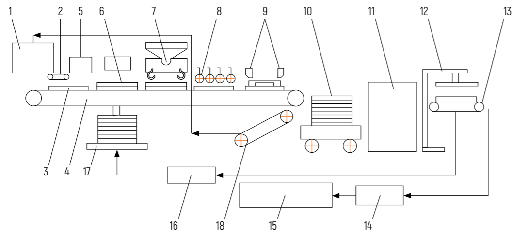
Figure 5 – Technological diagram of the pilot line for the production of glass concrete sheet elements: 1 – mixing unit; 2 – feeder-doser; 3 – mixture laying pallet; 4 – product molding conveyor; 5 – leveler; 6 – product molding pallet; 7 – tip-over device; 8 – vibration rollers; 9 – clippers; 10 – cart; 11 – prehardening chamber; 12 – demoulder; 13 – conveyor; 14 – wet hardening conveyor; 15 – finished product warehouse; 16 – pallet cleaning and lubrication station; 17 – relocater; 18 – mobile feed conveyor for primary materials
