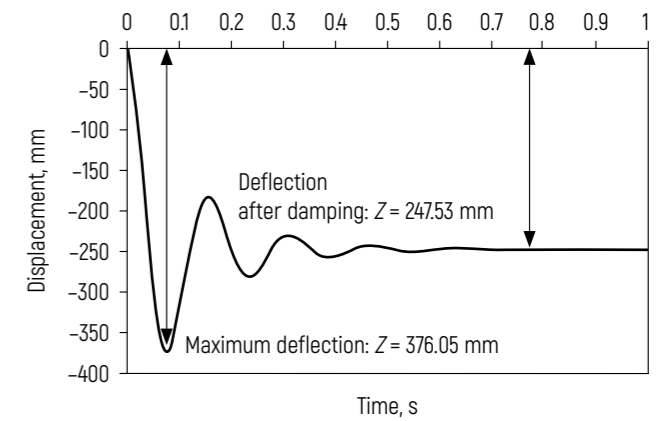
Figure 9 – Dynamic response of a cantilever beam loaded with a constant force
