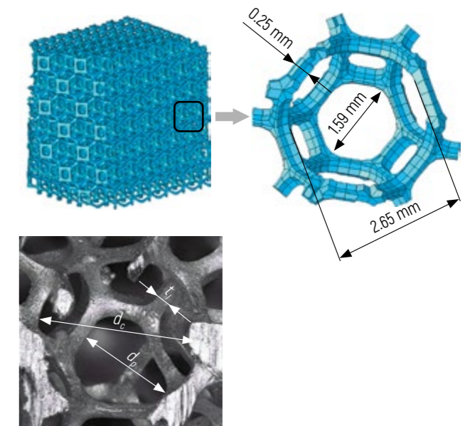
Figure 5 – Finite element model of foam aluminum with 40 ppi porosity
