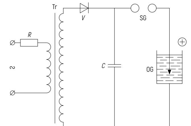
Figure 2 - A simplified wiring diagram of the UniThorr EHDE: R - charging resistor; Tr - transformer; V - rectifier; SG - shaping spark gap; OG - operating spark gap; C - operating capacitance of condenser
