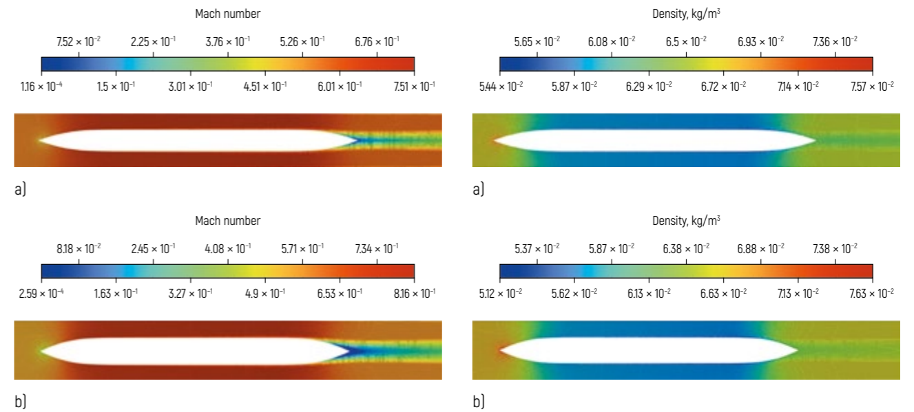
Figure 4 – Distribution of Mach number of methane gas medium in a forevacuum tunnel: a – for uPod fuselage diameter of 2 m and tunnel inner diameter of 5 m; b – for uPod fuselage diameter of 2.6 m and tunnel inner diameter of 6 m
