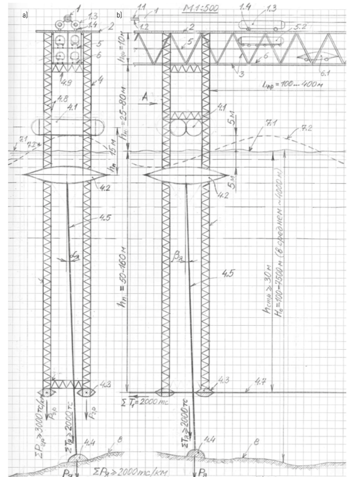
Figure 3 - Diagram of the GPV takeoff and landing overpass on oceanic section (option 2): a - cross section; b - side view
