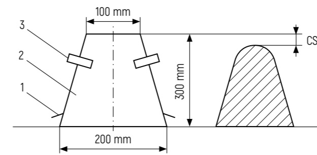
Figure 6 – Determination of mixture workability by cone sediment: 1 – supports; 2 – cone; 3 – handles; CS – cone sediment
