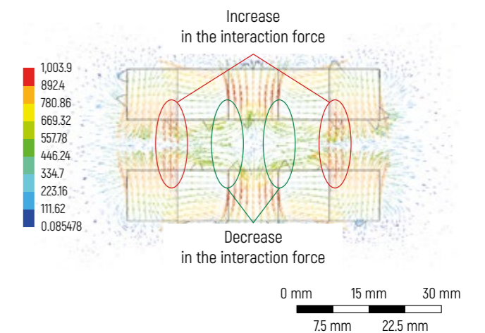
Figure 24 – 2D diagram of force vectors when plane neodymium magnets are used, mT
